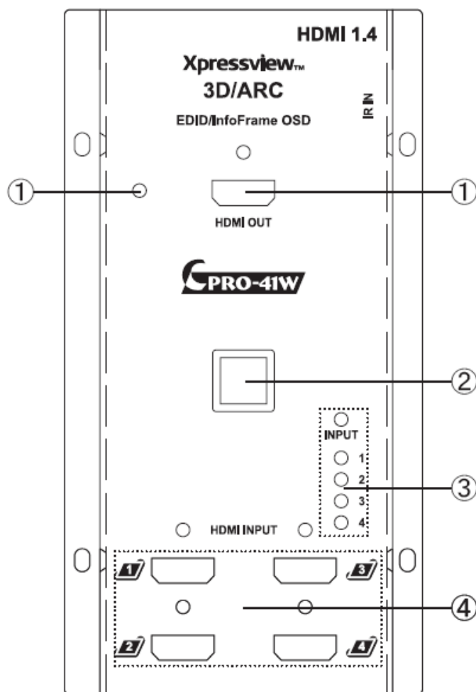
Front Panel
